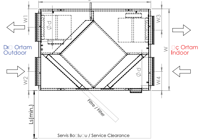
VHR 29/36/51
